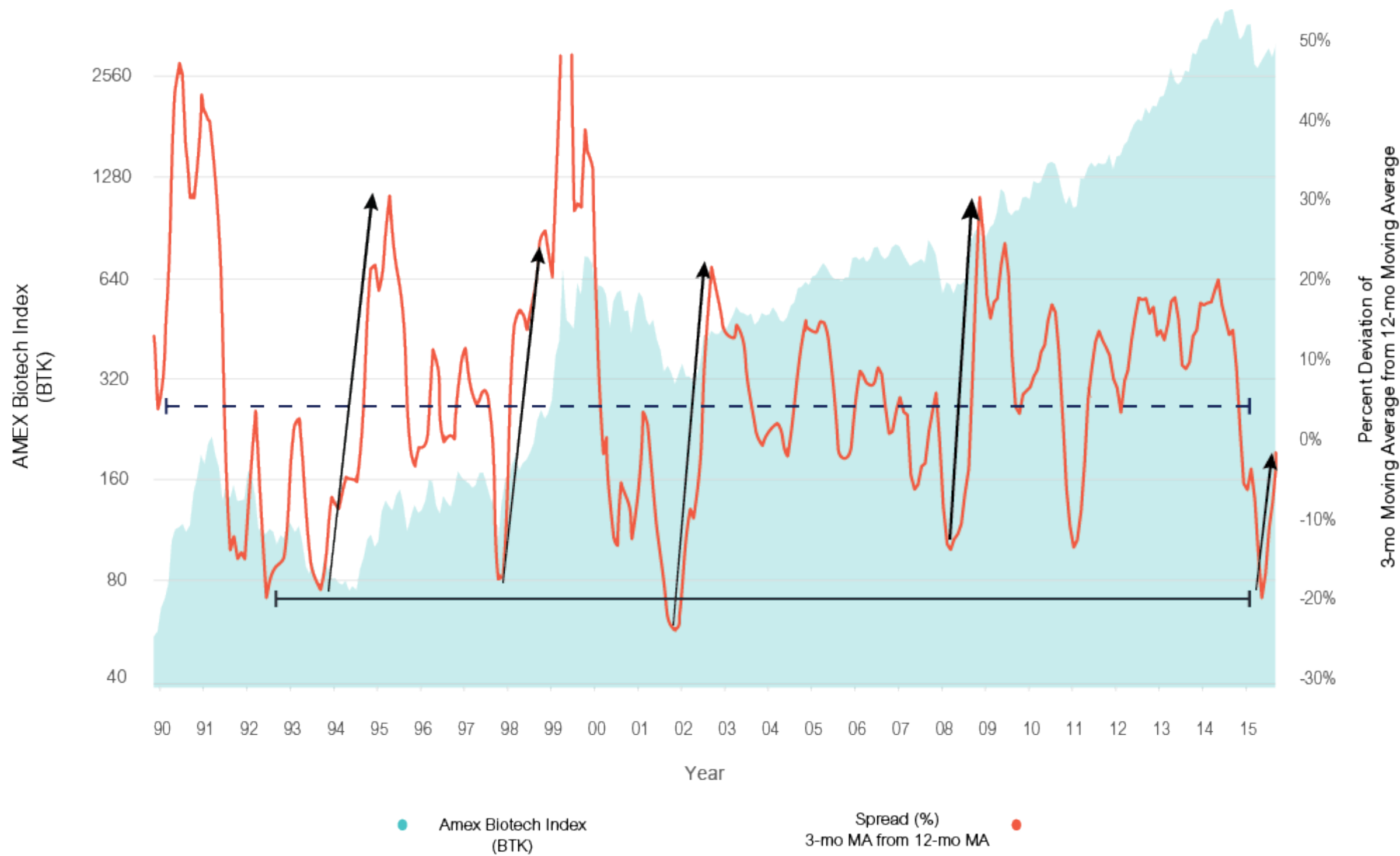
Signals: % Deviation of 3-month Minus 12-month Moving Average AMEX Biotech Index (BTK) 2015-2016
